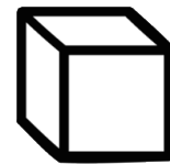
base 10 cube
